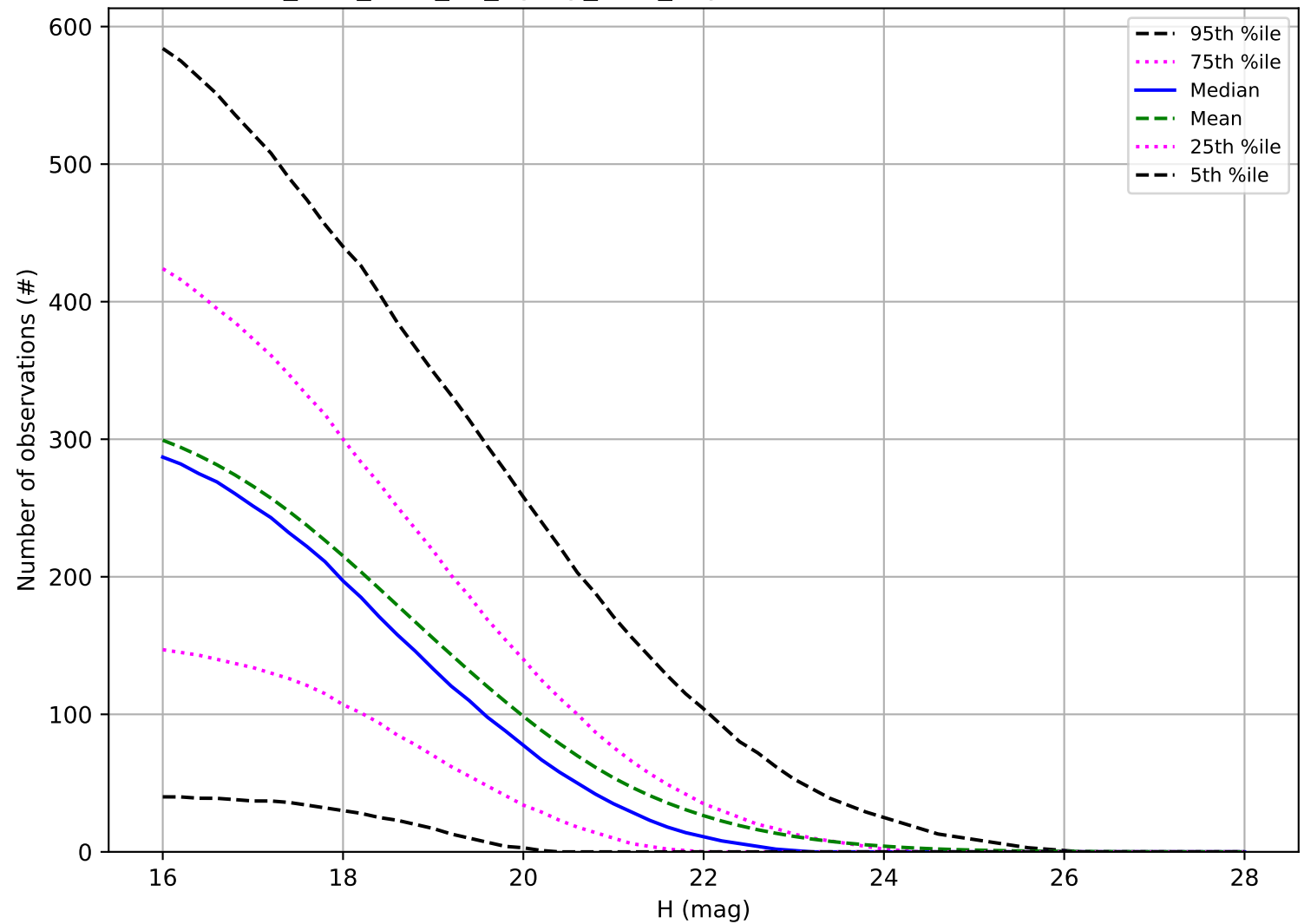
too_elab_r128_d3_ugrizy_v3.4_10yrs: Number of observations PHA
