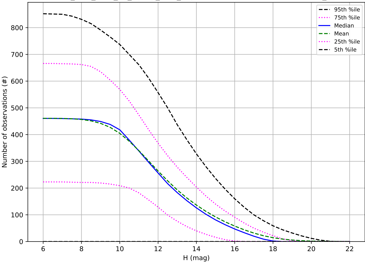
too_elab_r128_d3_ugrizy_v3.4_10yrs: Number of observations OCC_r5
