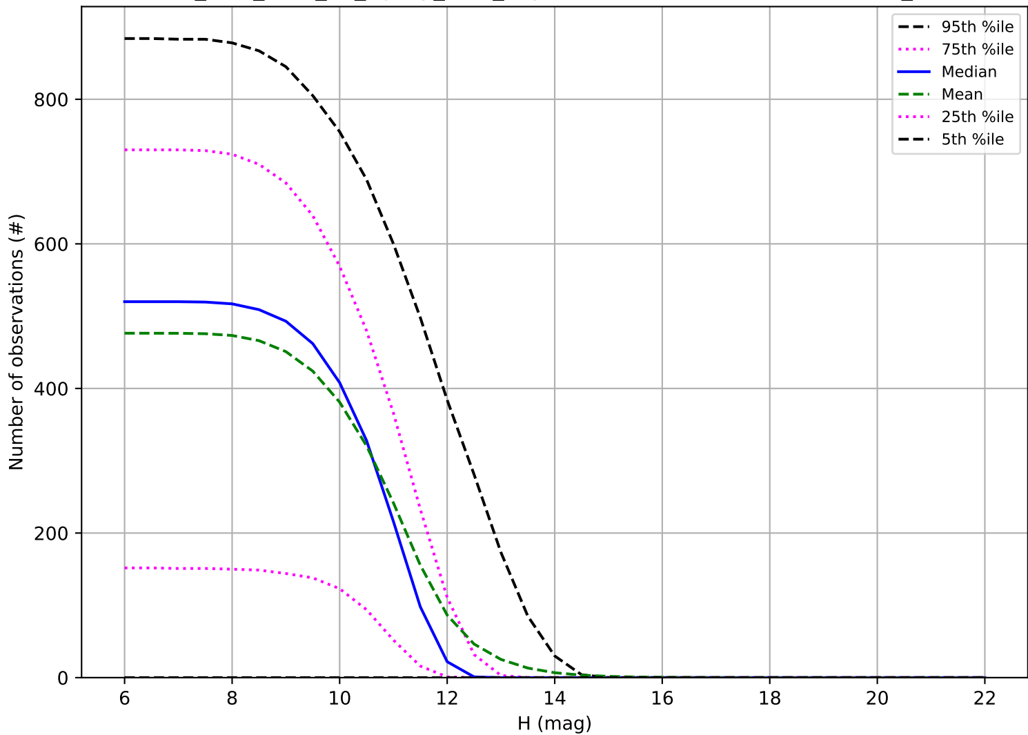
too_elab_r128_d3_ugrizy_v3.4_10yrs: Number of observations OCC_r20
