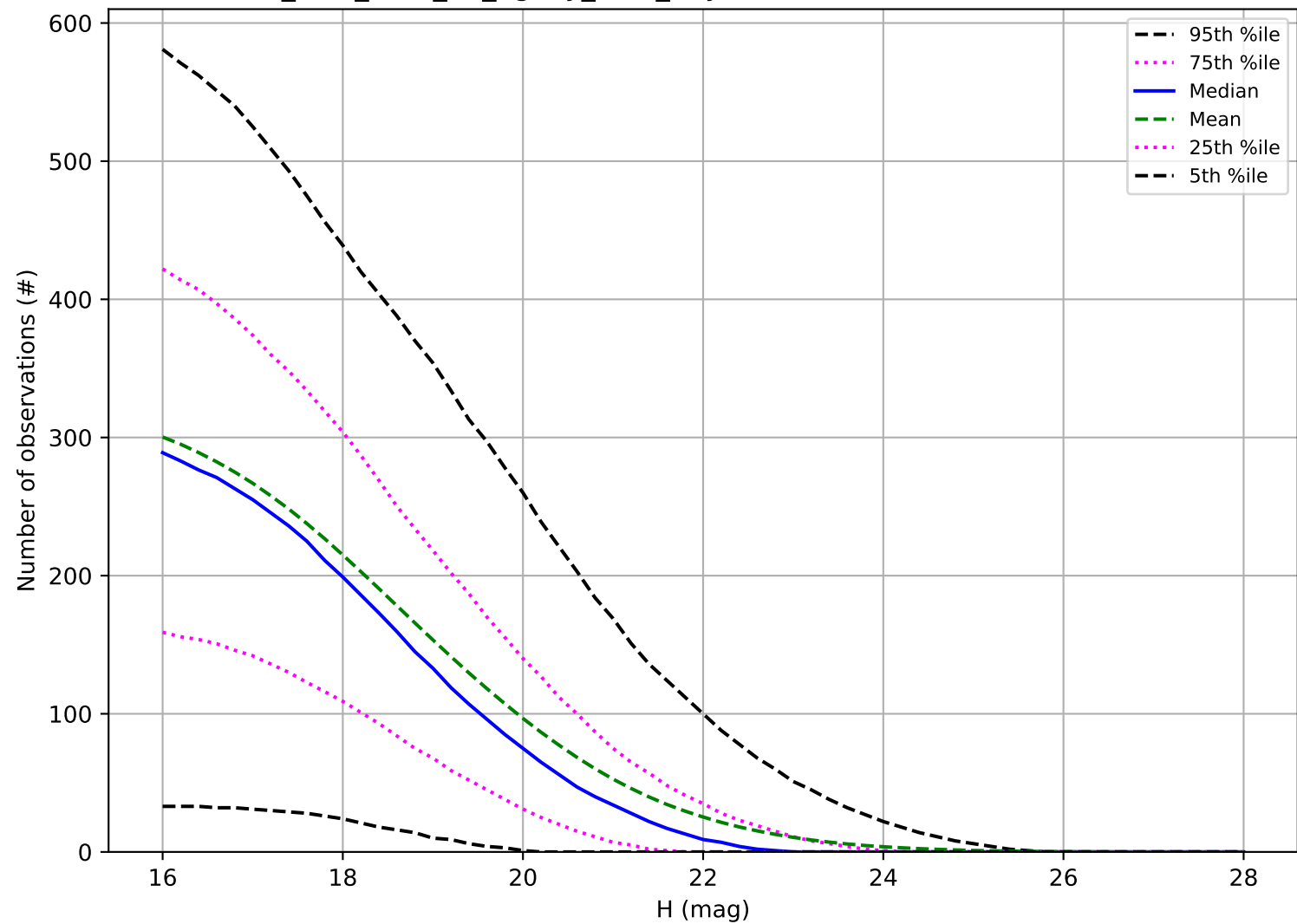
too_elab_r128_d3_ugrizy_v3.4_10yrs: Number of observations NEO
