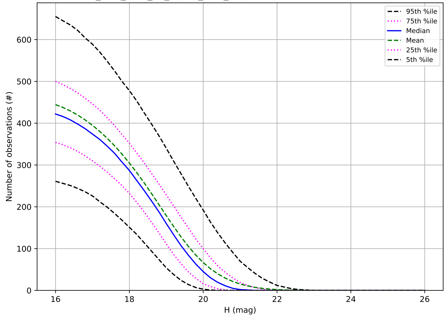
too_elab_r128_d3_ugrizy_v3.4_10yrs: Number of observations MBA
