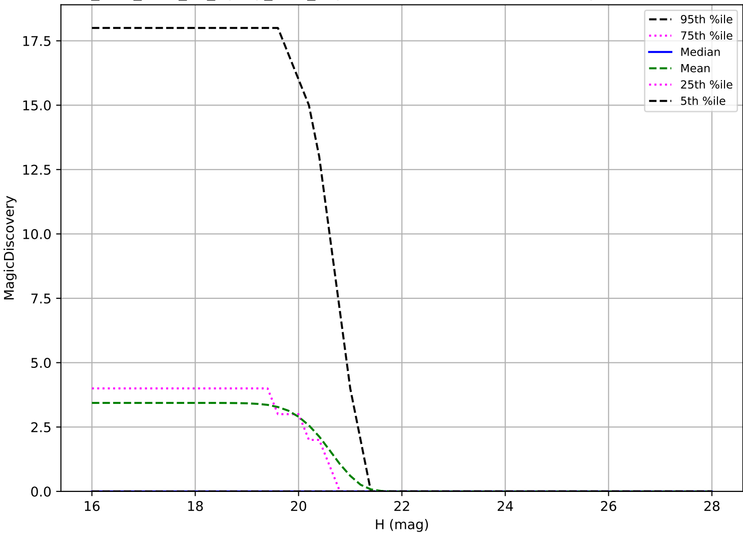
too_elab_r128_d3_ugrizy_v3.4_10yrs: Vatira 6 detections in 60 nights detection loss
