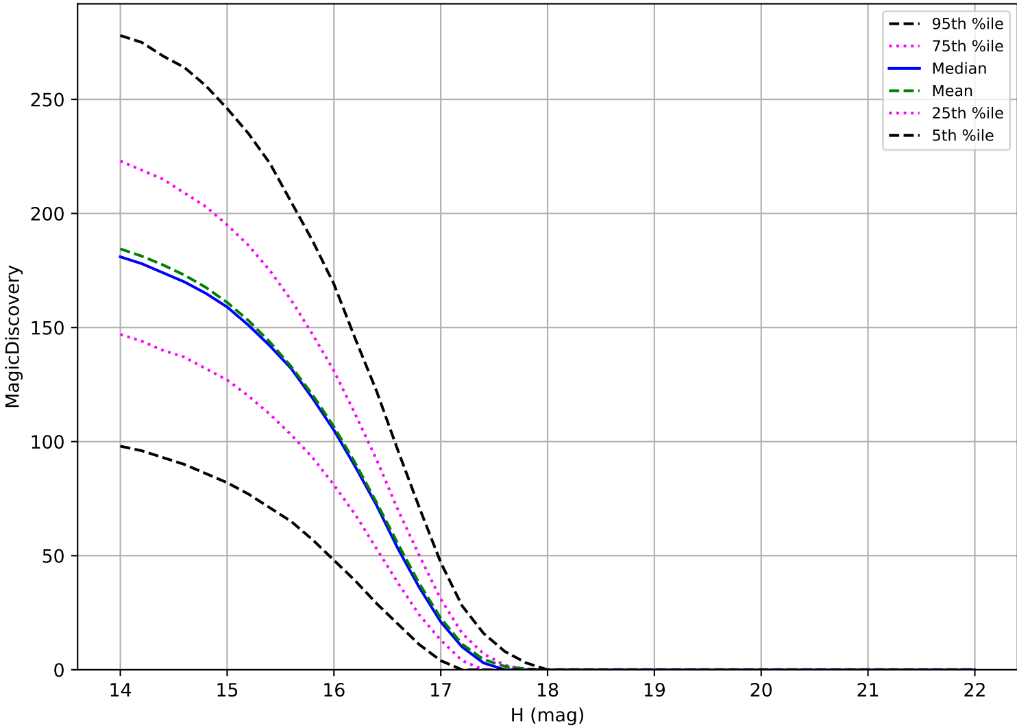
too_elab_r128_d3_ugrizy_v3.4_10yrs: Trojan 6 detections in 60 nights detection loss
