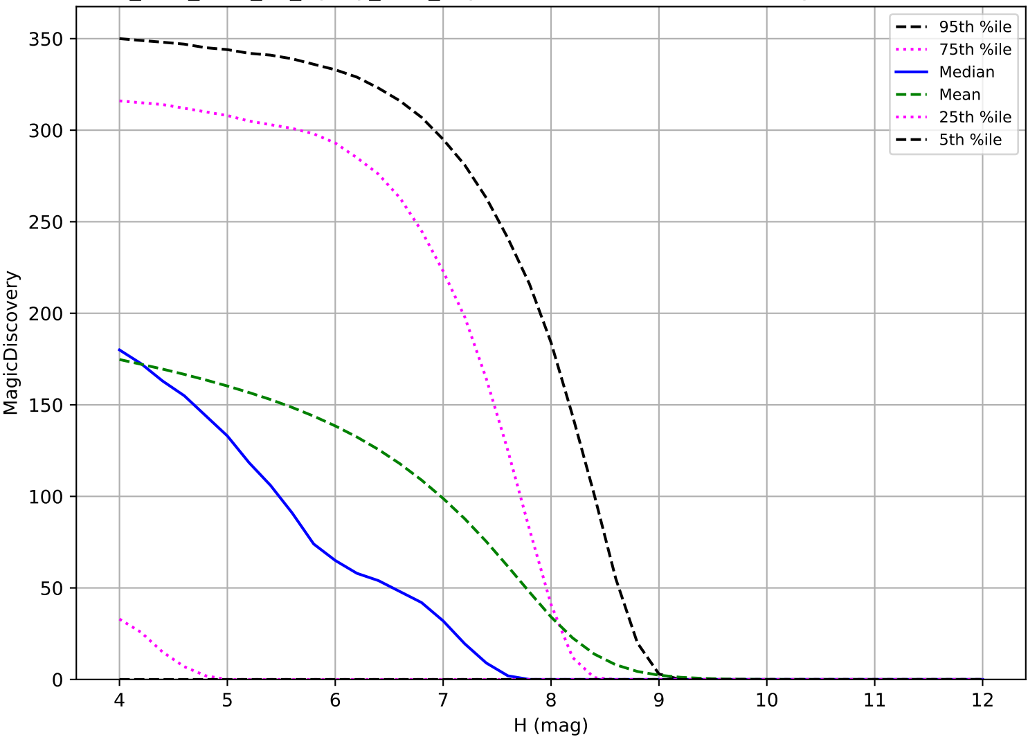
too_elab_r128_d3_ugrizy_v3.4_10yrs: TNO 6 detections in 60 nights detection loss
