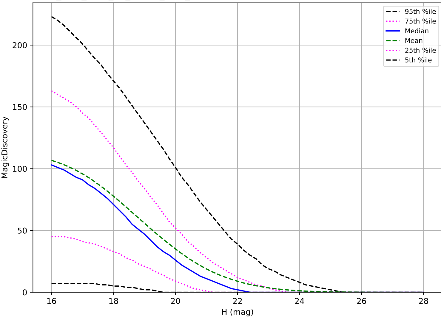
too_elab_r128_d3_ugrizy_v3.4_10yrs: PHA 6 detections in 60 nights detection loss
