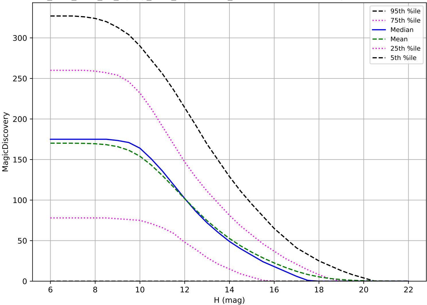
too_elab_r128_d3_ugrizy_v3.4_10yrs: OCC_r5 6 detections in 60 nights detection loss
