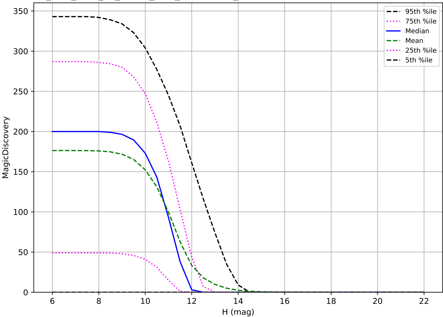
too_elab_r128_d3_ugrizy_v3.4_10yrs: OCC_r20 6 detections in 60 nights detection loss
