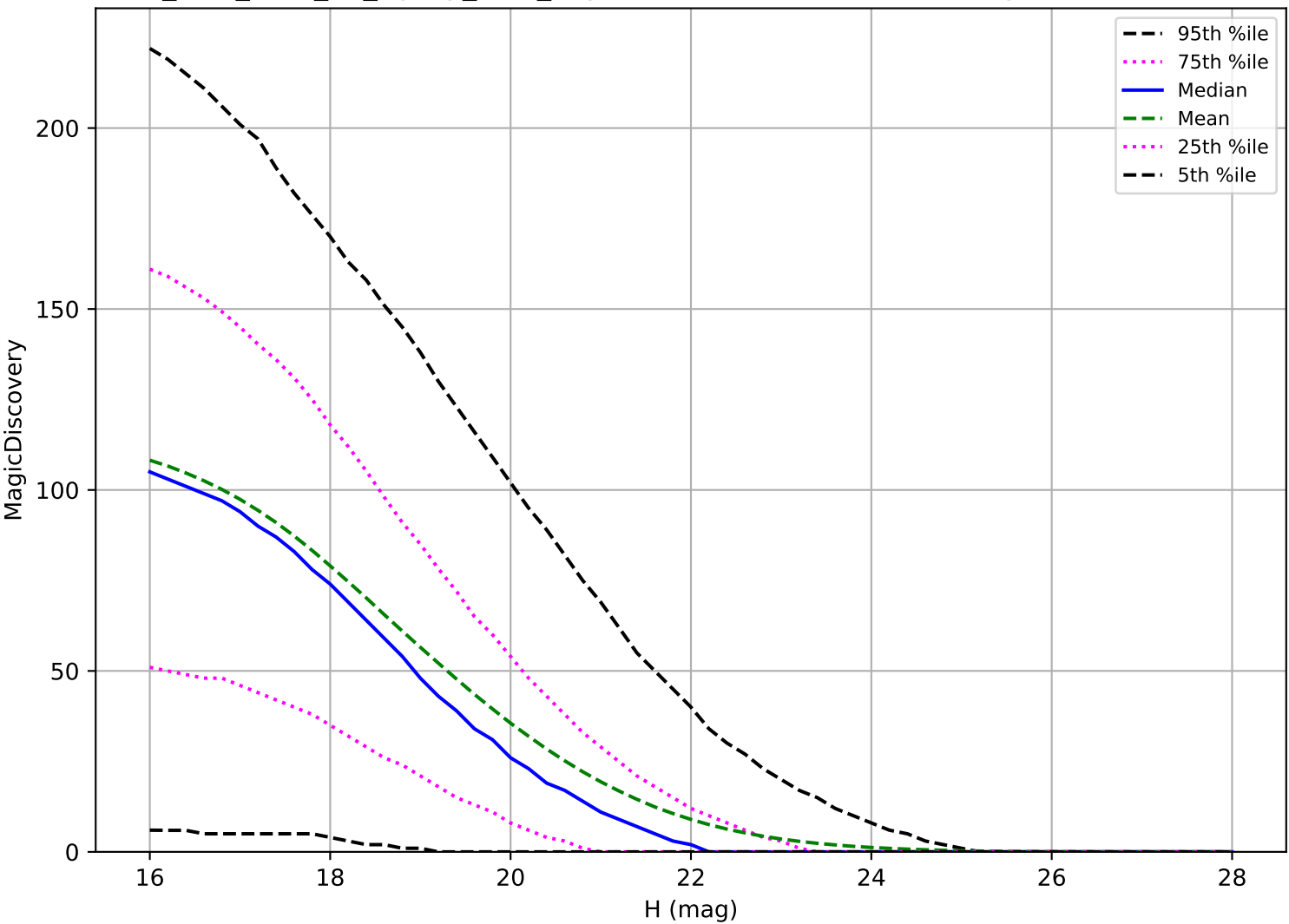
too_elab_r128_d3_ugrizy_v3.4_10yrs: NEO 6 detections in 60 nights detection loss
