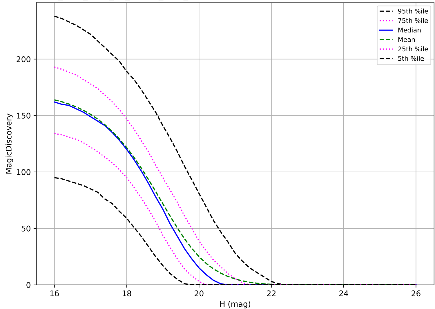
too_elab_r128_d3_ugrizy_v3.4_10yrs: MBA 6 detections in 60 nights detection loss
