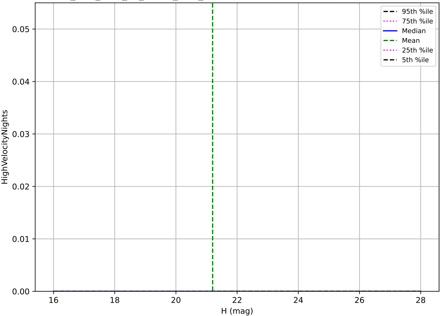
too_elab_r128_d3_ugrizy_v3.4_10yrs: Vatira High velocity pair detection loss
