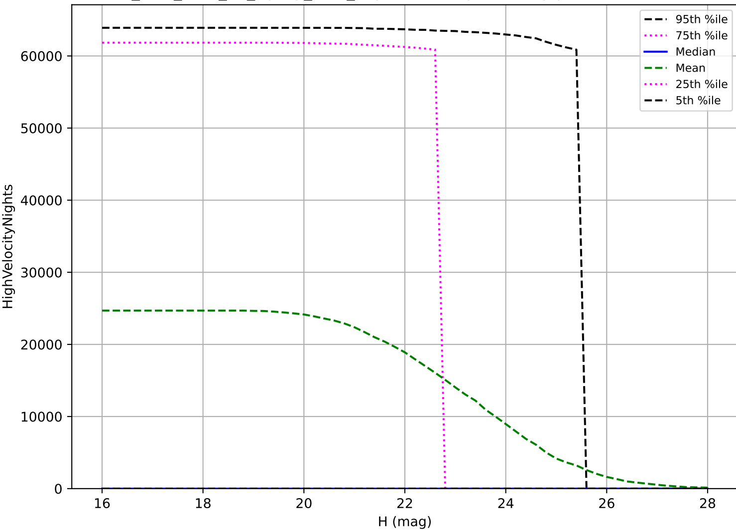
too_elab_r128_d3_ugrizy_v3.4_10yrs: PHA High velocity pair detection loss
