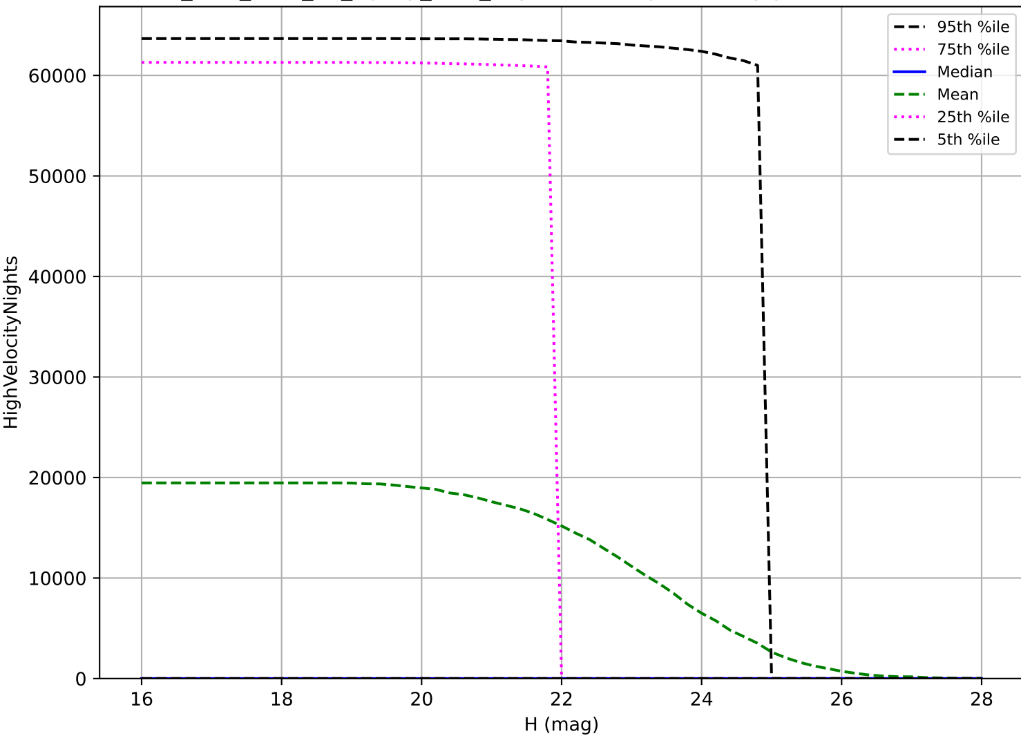
too_elab_r128_d3_ugrizy_v3.4_10yrs: NEO High velocity pair detection loss
