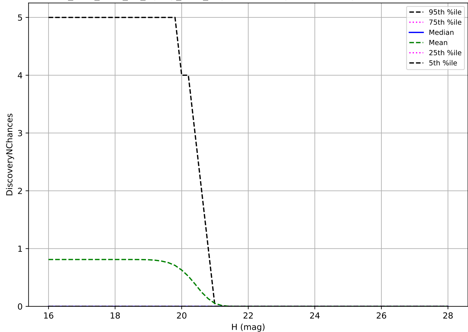
too_elab_r128_d3_ugrizy_v3.4_10yrs: Vatira 3 pairs in 15 nights detection loss
