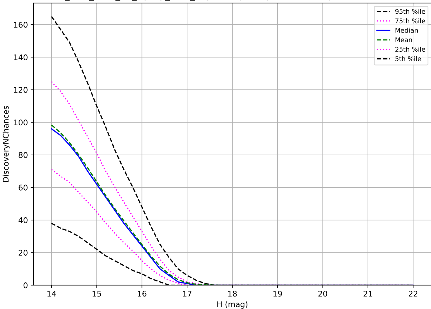
too_elab_r128_d3_ugrizy_v3.4_10yrs: Trojan 3 pairs in 15 nights detection loss
