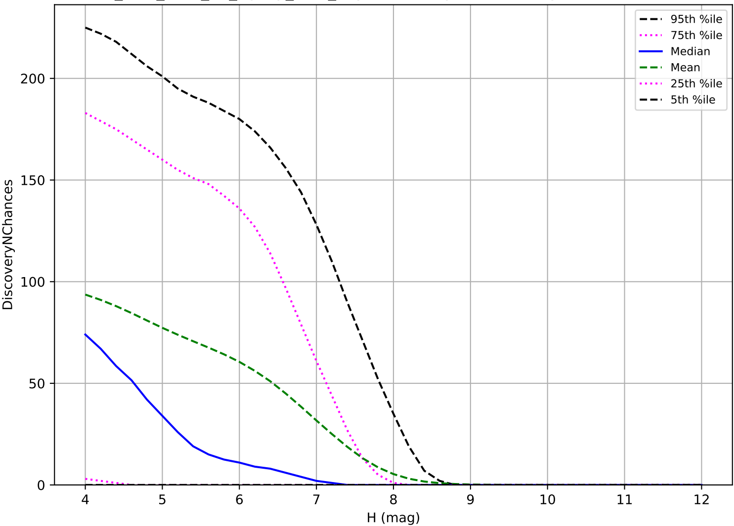
too_elab_r128_d3_ugrizy_v3.4_10yrs: TNO 3 pairs in 15 nights detection loss
