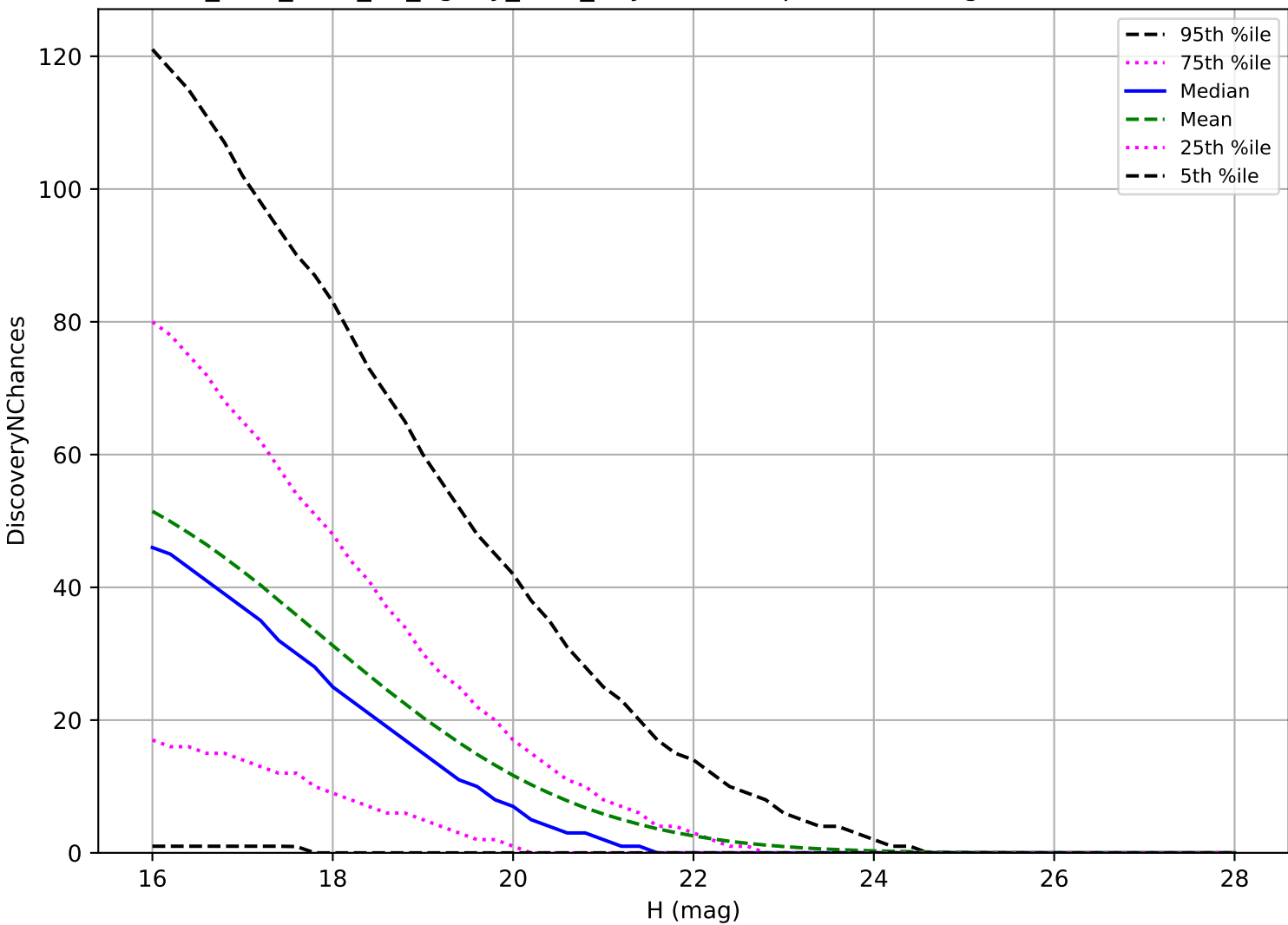
too_elab_r128_d3_ugrizy_v3.4_10yrs: PHA 3 pairs in 15 nights detection loss
