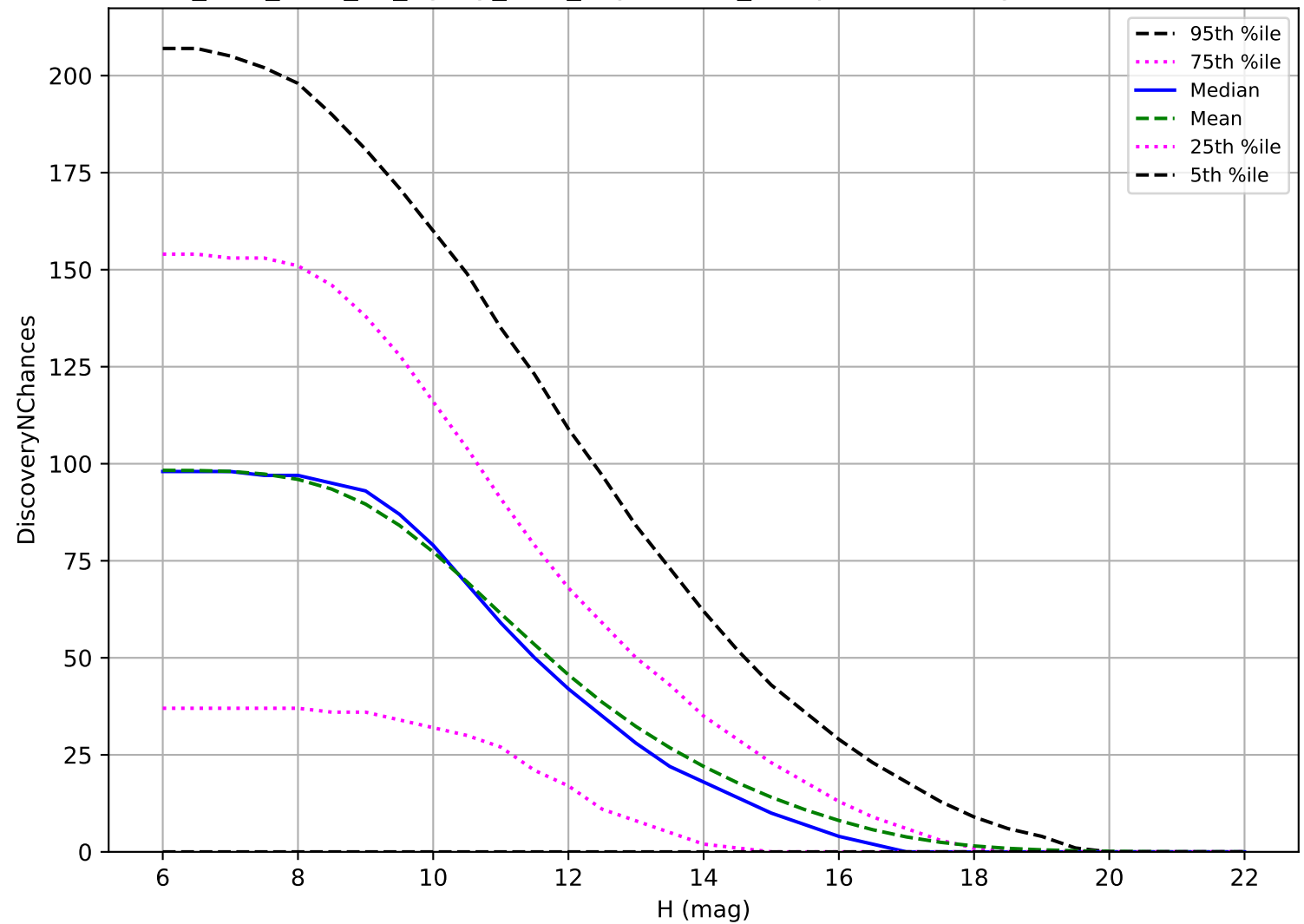
too_elab_r128_d3_ugrizy_v3.4_10yrs: OCC_r5 3 pairs in 15 nights detection loss
