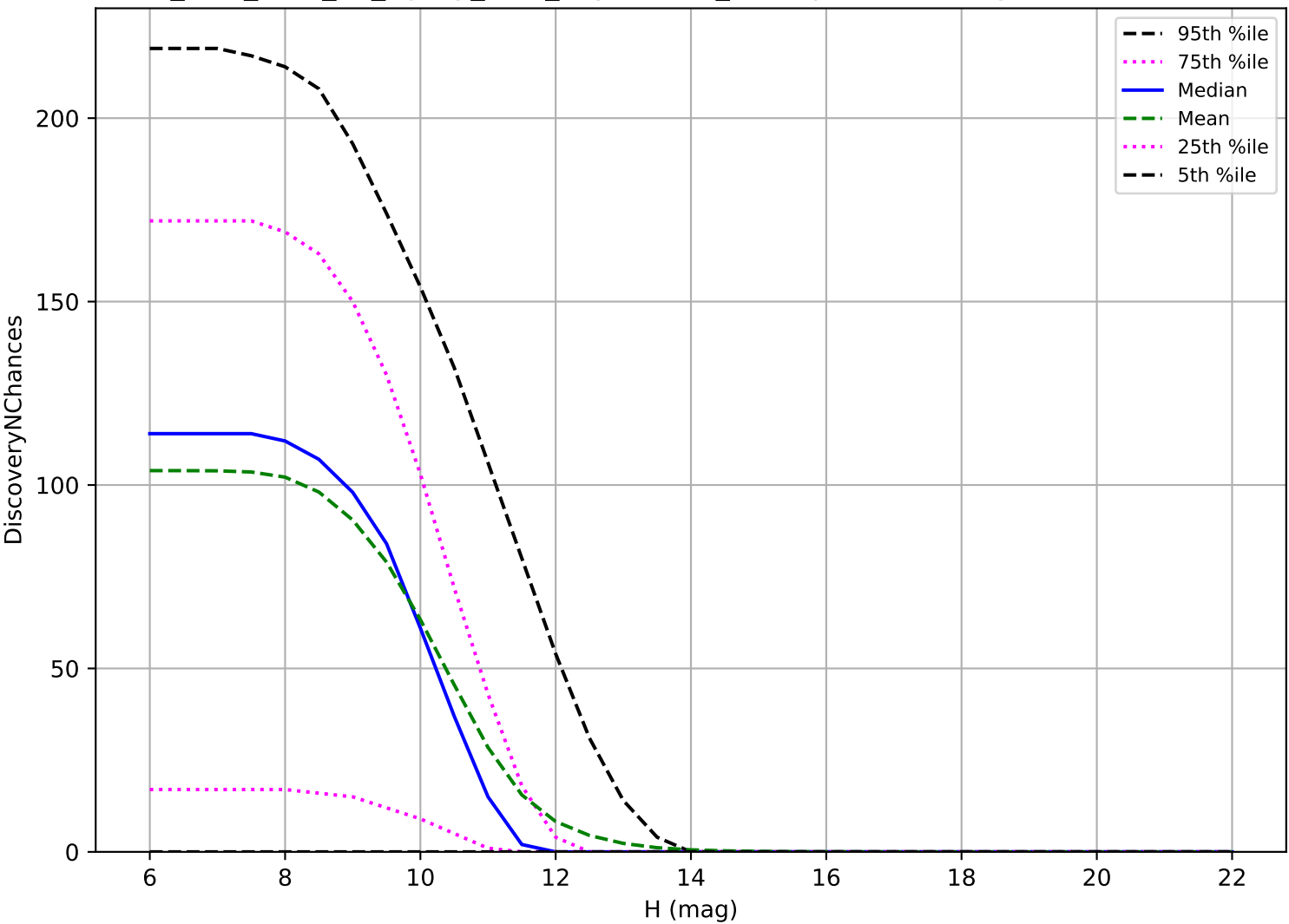
too_elab_r128_d3_ugrizy_v3.4_10yrs: OCC_r20 3 pairs in 15 nights detection loss
