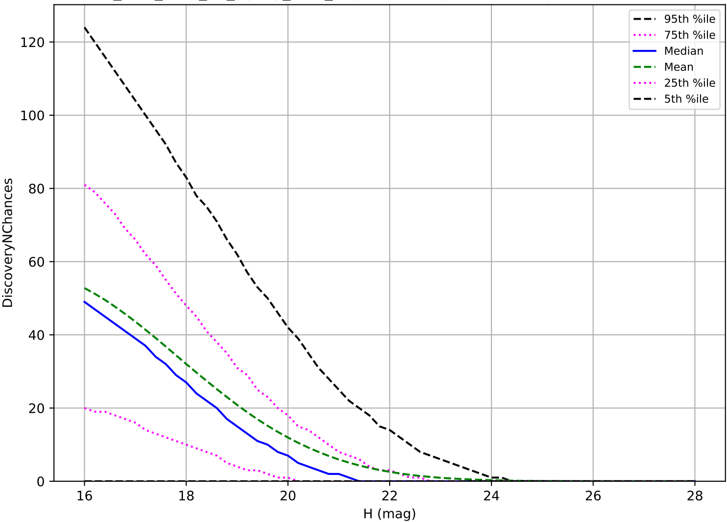
too_elab_r128_d3_ugrizy_v3.4_10yrs: NEO 3 pairs in 15 nights detection loss
