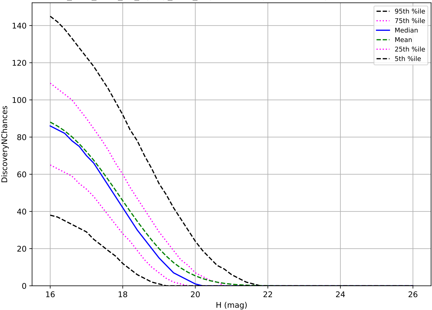
too_elab_r128_d3_ugrizy_v3.4_10yrs: MBA 3 pairs in 15 nights detection loss
