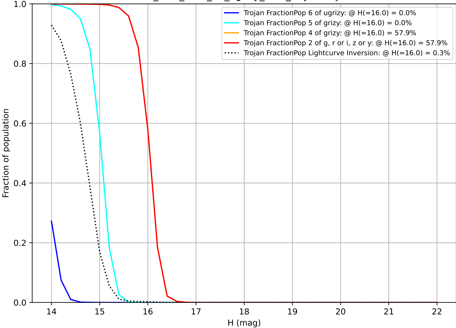
too_elab_r128_d3_ugrizy_v3.4_10yrs Trojan
