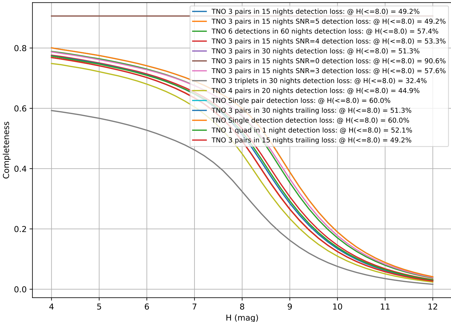
too_elab_r128_d3_ugrizy_v3.4_10yrs: CumulativeCompleteness
