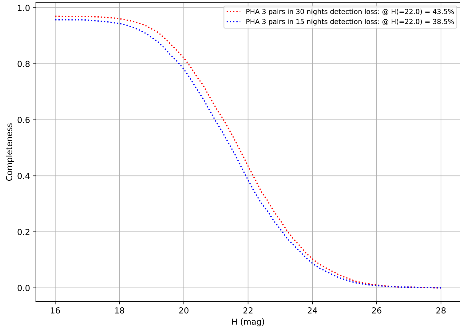
too_elab_r128_d3_ugrizy_v3.4_10yrs: DifferentialCompleteness
