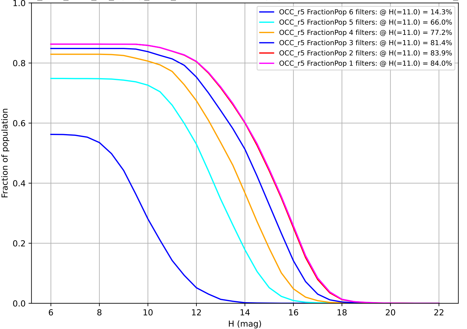
too_elab_r128_d3_ugrizy_v3.4_10yrs: Fraction of population with colors in X filters OCC_r5
