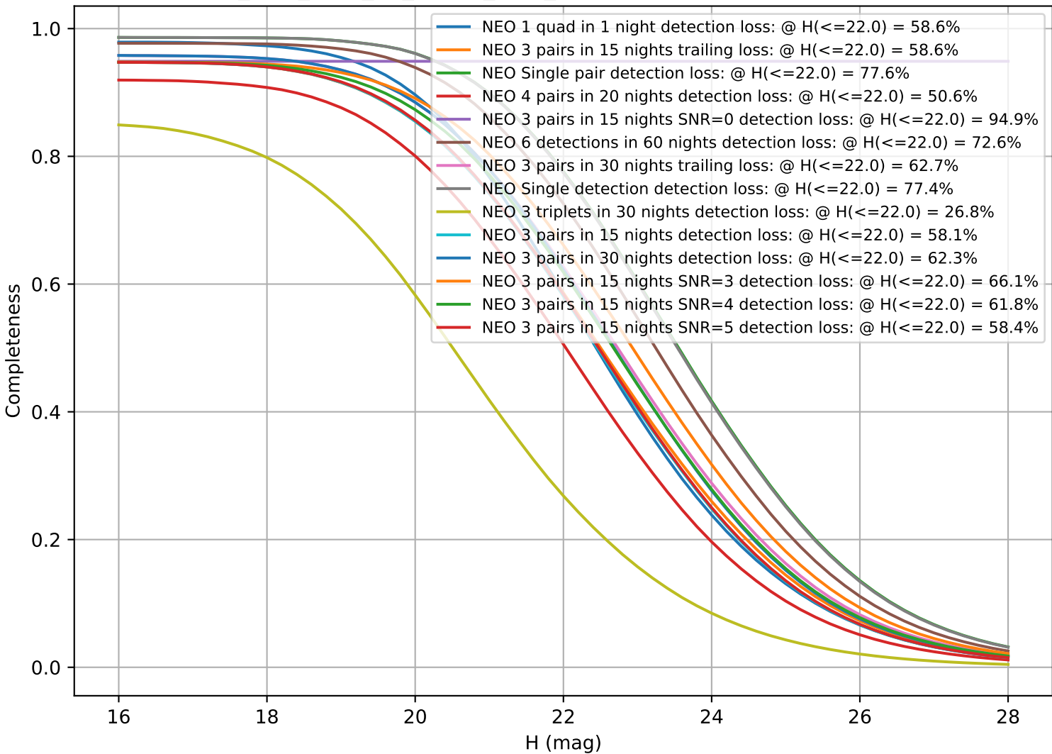
too_elab_r128_d3_ugrizy_v3.4_10yrs: CumulativeCompleteness
