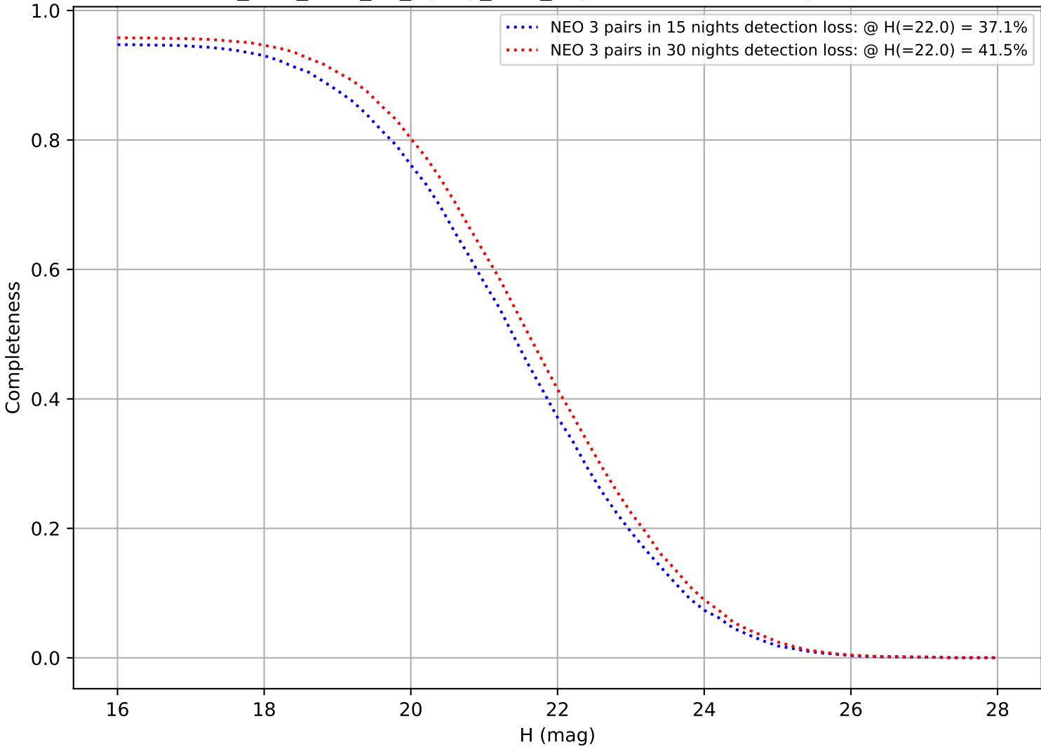
too_elab_r128_d3_ugrizy_v3.4_10yrs: DifferentialCompleteness
