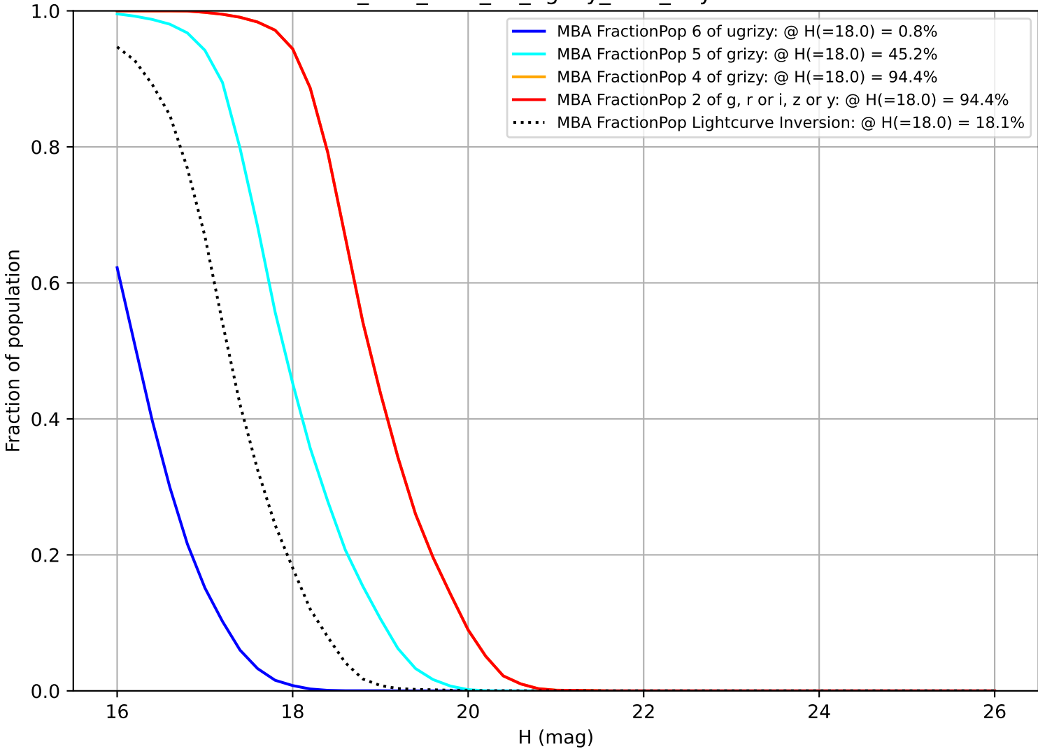
too_elab_r128_d3_ugrizy_v3.4_10yrs MBA
