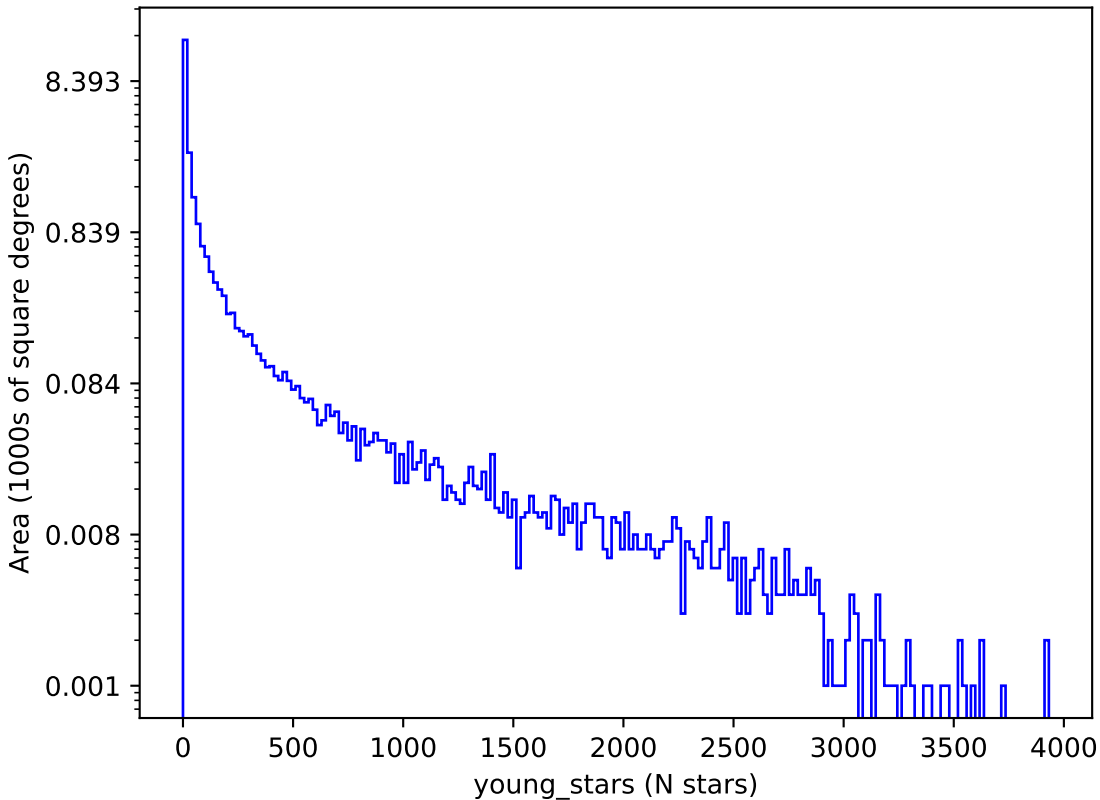
too_elab_r128_d3_ugrizy_v3.4_10yrs : young_stars
