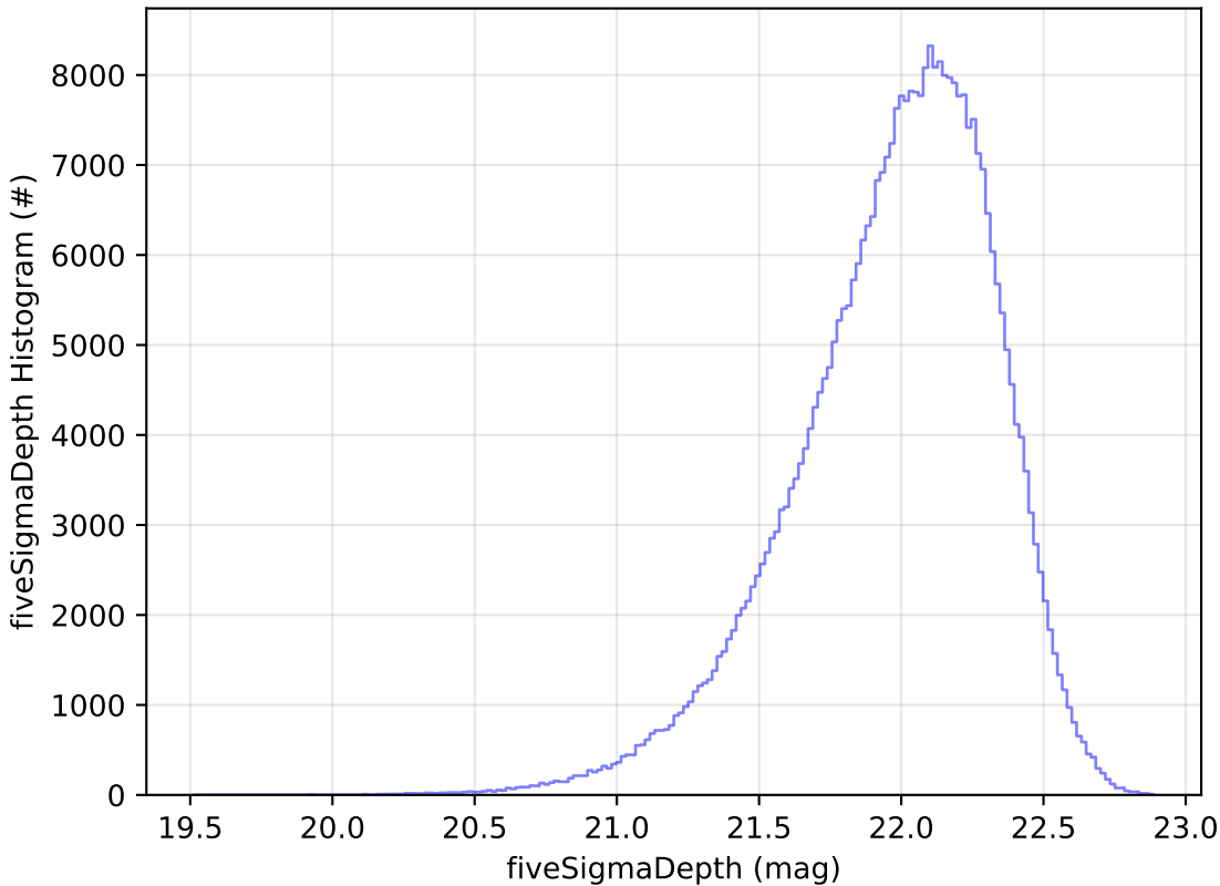
too_elab_r128_d3_ugrizy_v3.4_10yrs y: fiveSigmaDepth Histogram
