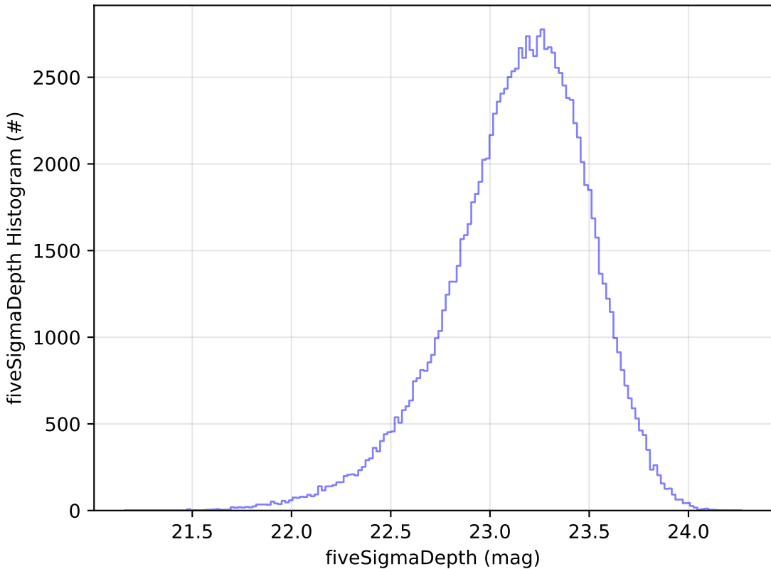
too_elab_r128_d3_ugrizy_v3.4_10yrs u: fiveSigmaDepth Histogram
