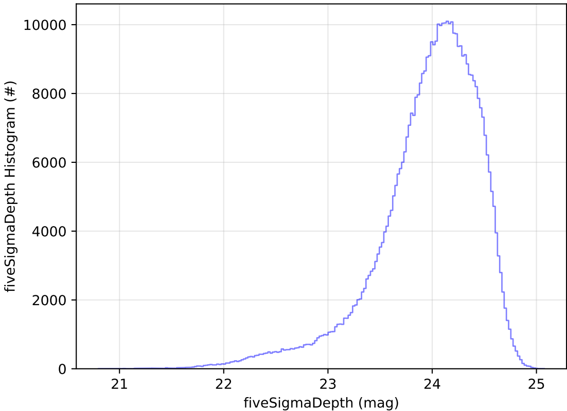
too_elab_r128_d3_ugrizy_v3.4_10yrs r: fiveSigmaDepth Histogram
