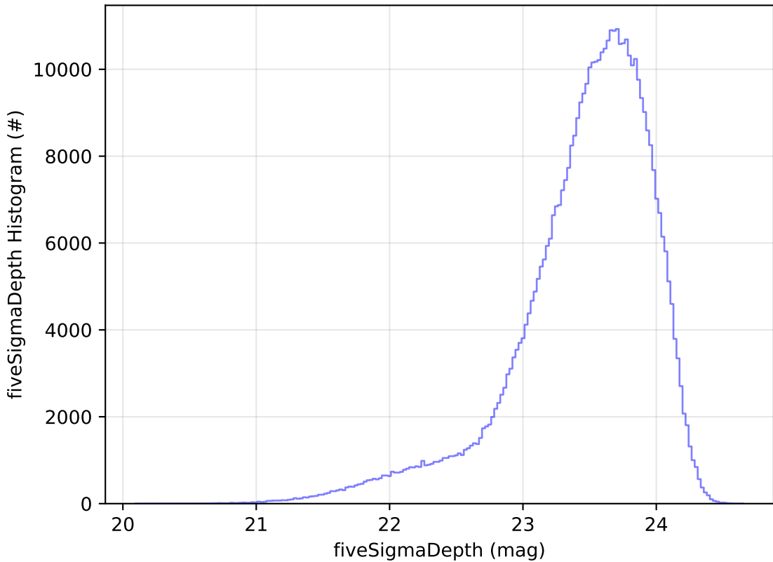
too_elab_r128_d3_ugrizy_v3.4_10yrs i: fiveSigmaDepth Histogram
