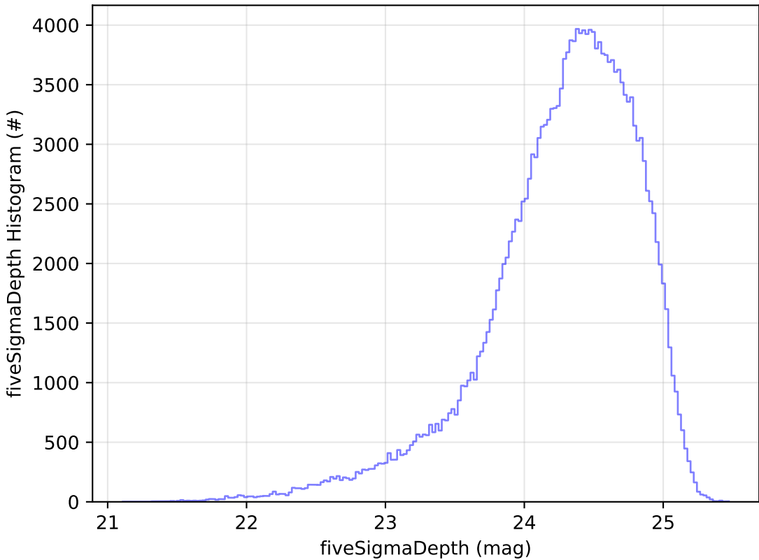
too_elab_r128_d3_ugrizy_v3.4_10yrs g: fiveSigmaDepth Histogram
