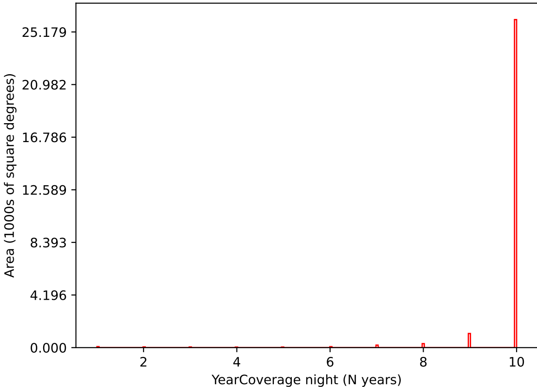
too_elab_r128_d3_ugrizy_v3.4_10yrs i band: YearCoverage night
