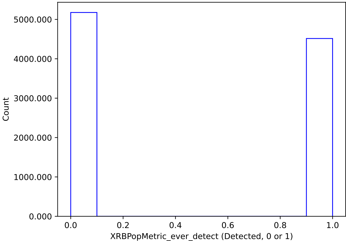
too_elab_r128_d3_ugrizy_v3.4_10yrs : XRBPopMetric_ever_detect
