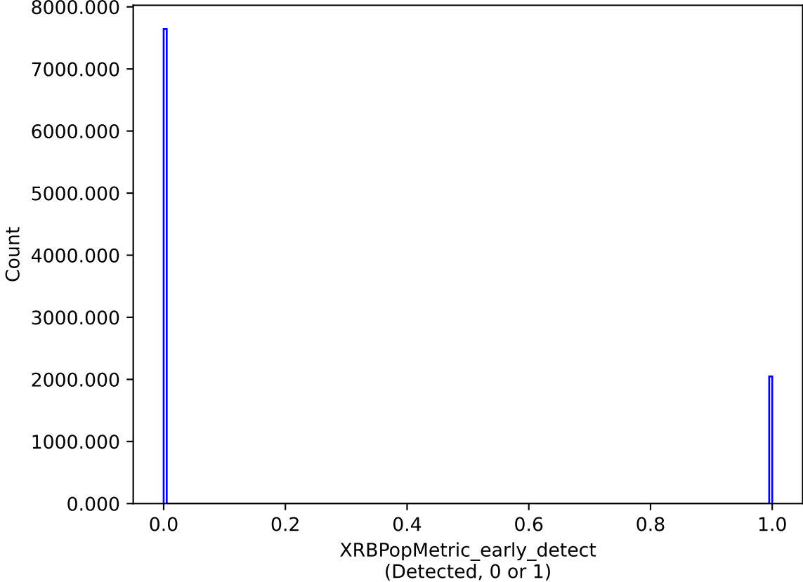
too_elab_r128_d3_ugrizy_v3.4_10yrs : XRBPopMetric_early_detect
