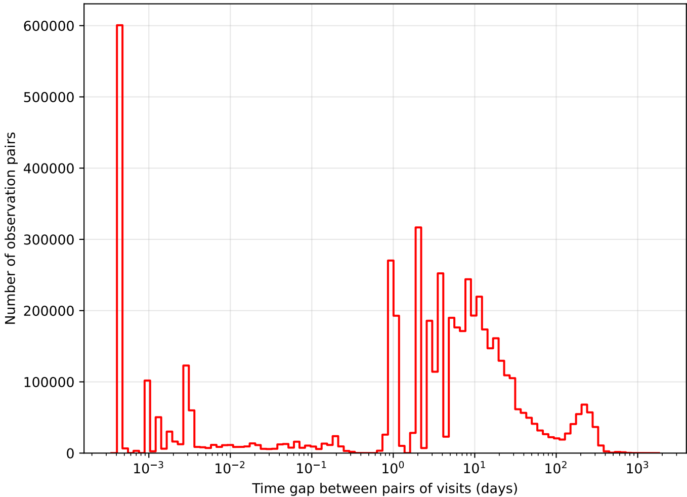
too_elab_r128_d3_ugrizy_v3.4_10yrs i band: Tgaps observationStartMJD
