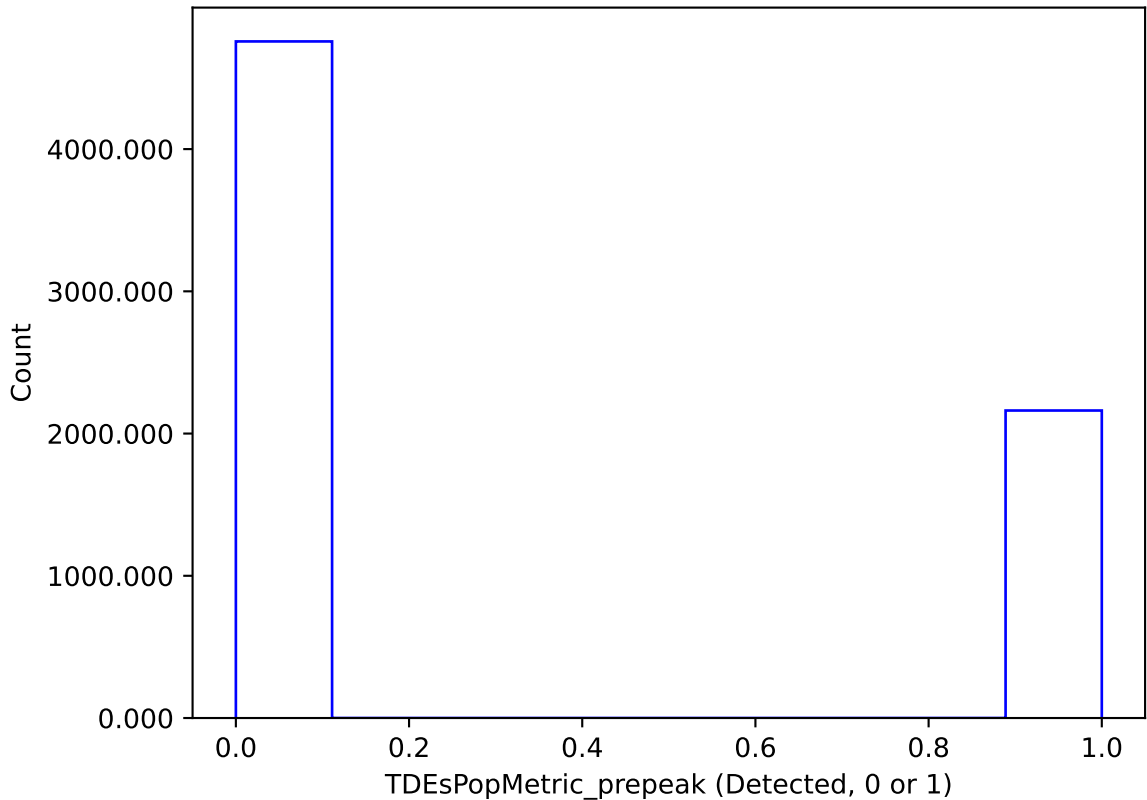
too_elab_r128_d3_ugrizy_v3.4_10yrs : TDEsPopMetric_prepeak
