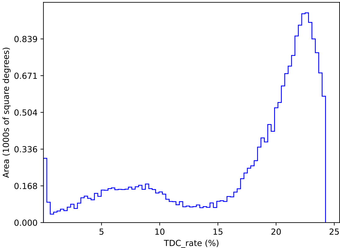
too_elab_r128_d3_ugrizy_v3.4_10yrs : TDC_rate
