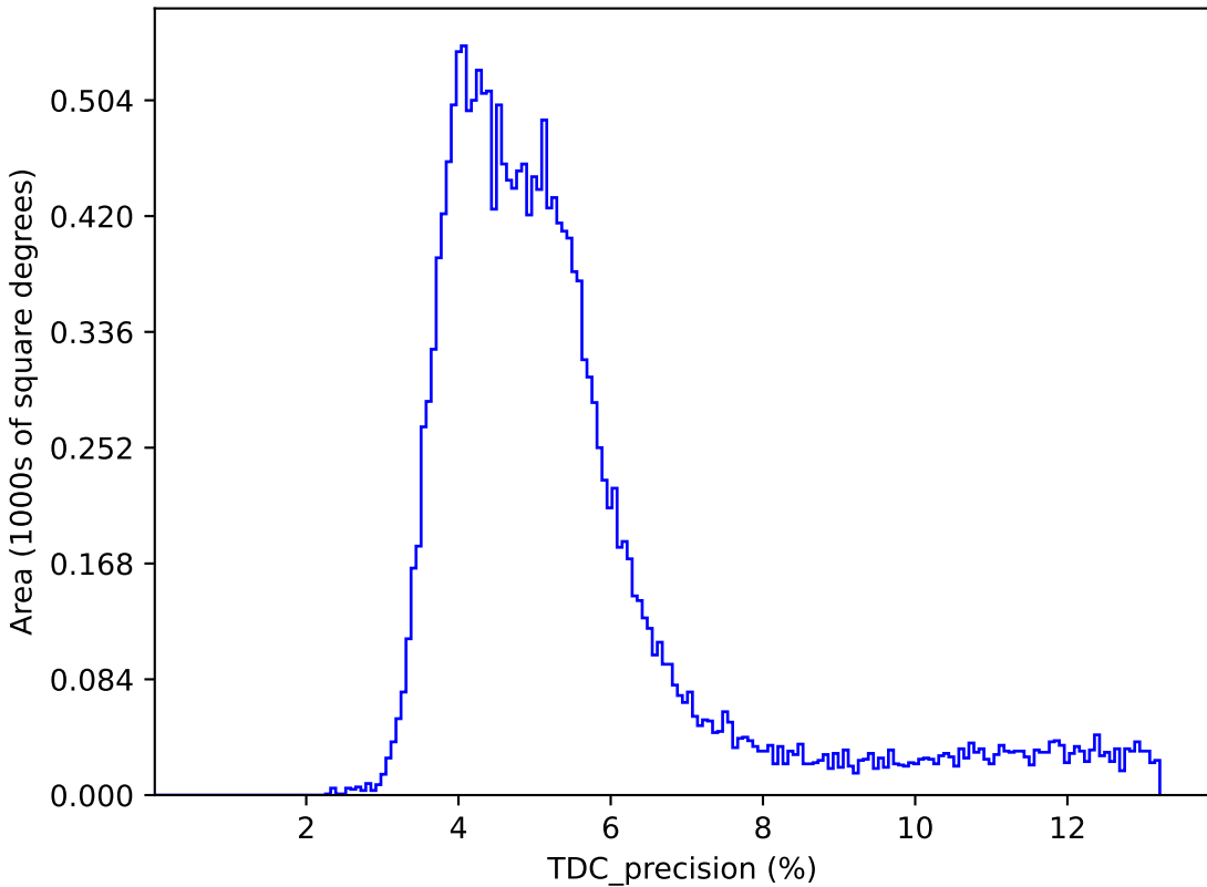
too_elab_r128_d3_ugrizy_v3.4_10yrs : TDC_precision
