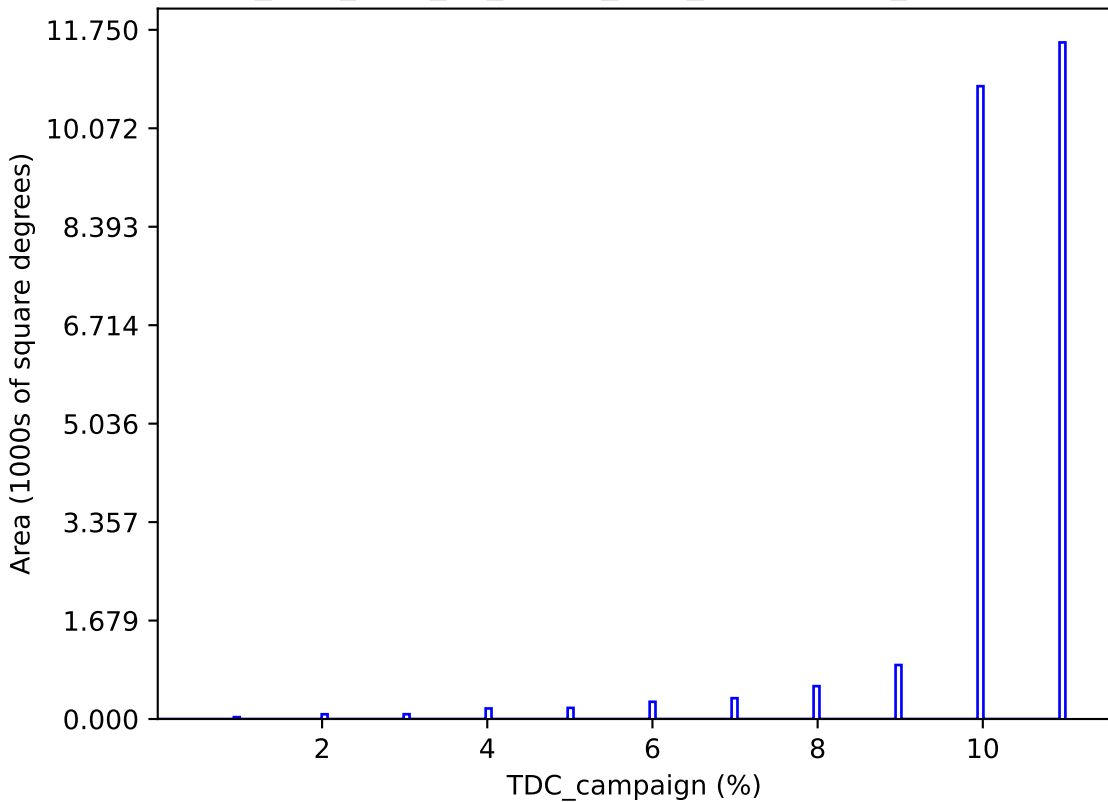
too_elab_r128_d3_ugrizy_v3.4_10yrs : TDC_campaign
