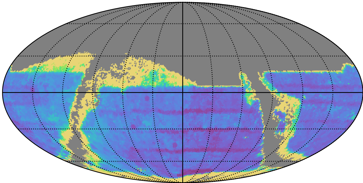
too_elab_r128_d3_ugrizy_v3.4_10yrs : TDC_accuracy
