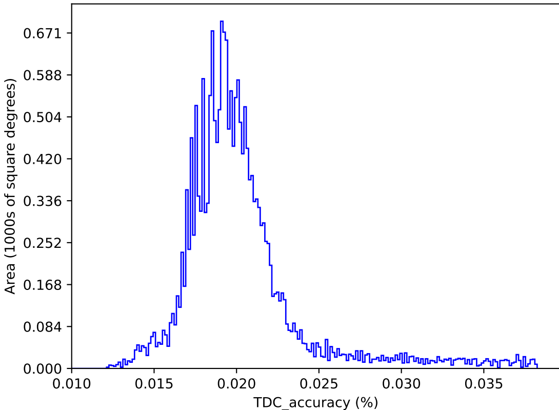
too_elab_r128_d3_ugrizy_v3.4_10yrs : TDC_accuracy
