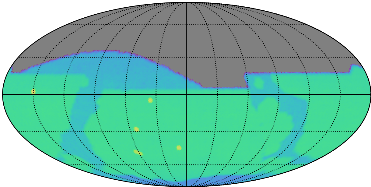
too_elab_r128_d3_ugrizy_v3.4_10yrs i: SurfaceBrightLimit
