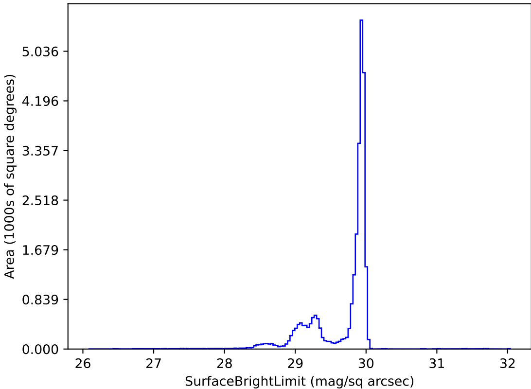
too_elab_r128_d3_ugrizy_v3.4_10yrs i: SurfaceBrightLimit
