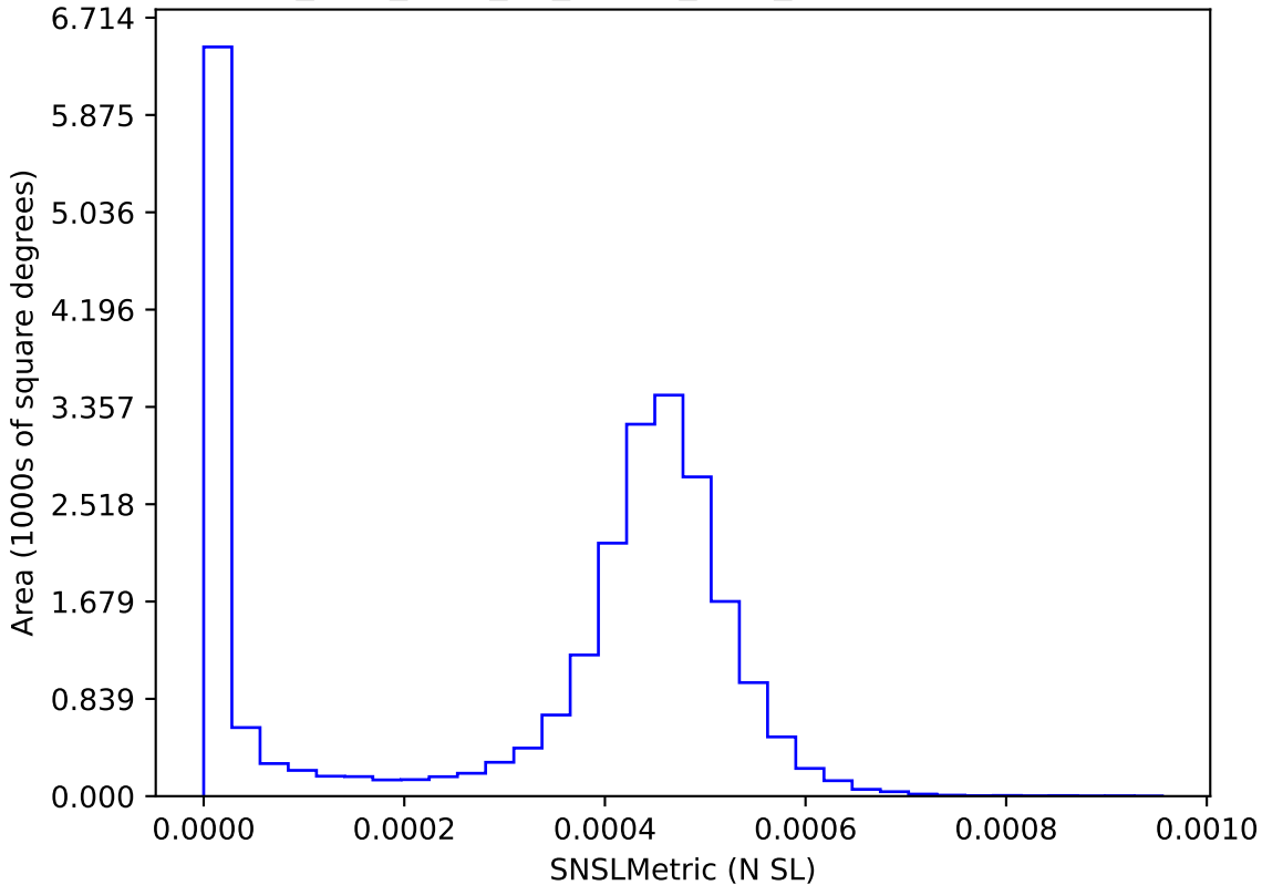
too_elab_r128_d3_ugrizy_v3.4_10yrs : SNSLMetric
